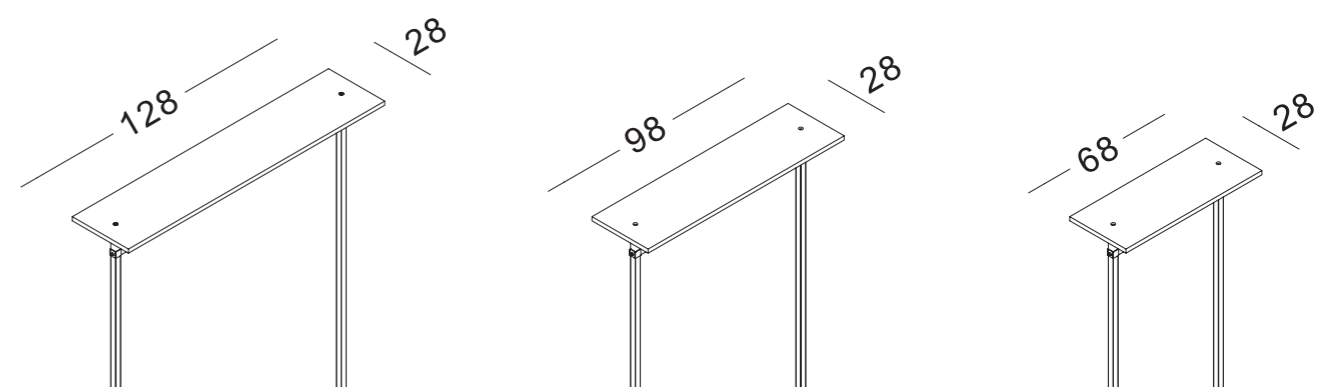
RBWM1 mensola per RBW1-4-C-B shelves for RBW1-4-C-B
