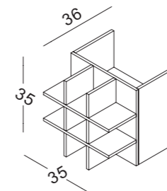
RBWAP3 casellario cravatte per RBWAP7-8-9 tie holder for RBWAP7-8-9
